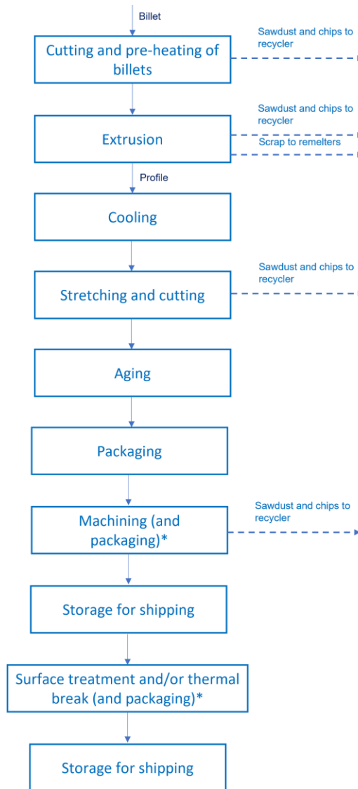
Figure 1: Production process of the aluminium profile 6063, produced in Borgo Valbelluna and Feltre by Pandolfo Alluminio. * Added value works can be performed in several order (e.g. anodising and then machining, or viceversa).
